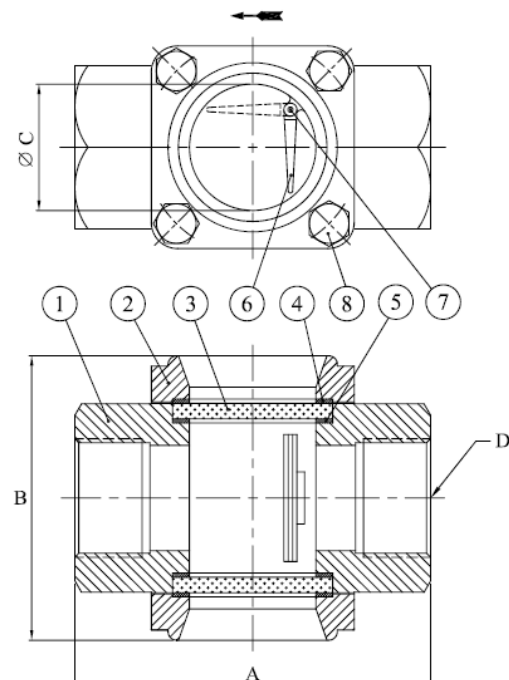
DN 1"1/4 to 2"
