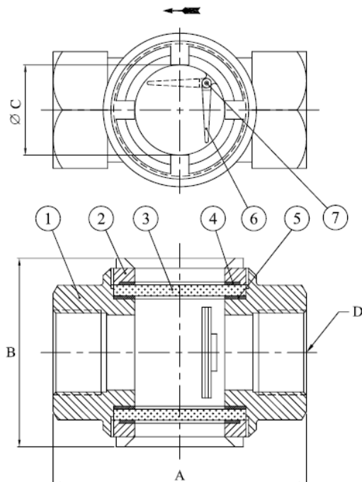
DN 1/2" to 1"
